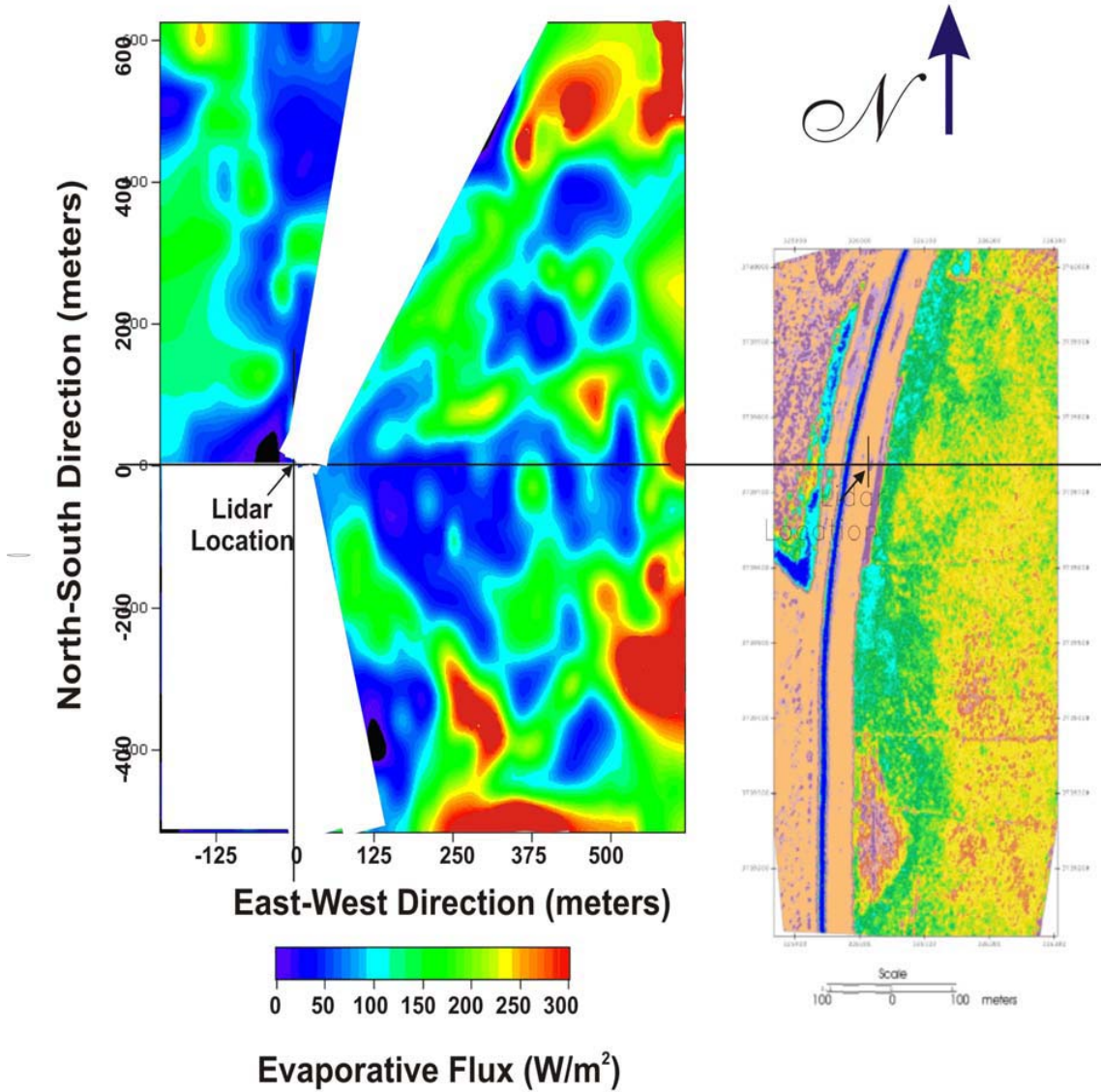
Figure 2. An evaporation map (left) of the Bosque del Apache site; reds are highest rates, blues lowest. To the right is a thermal infrared aerial photograph; reds are warmest, blues are cool. The two plots show the lidar location, are to the same scale, and are aligned horizontally for ease of comparison. The canopy to the east of the lidar is salt cedar and to the north west are cottonwood trees.
