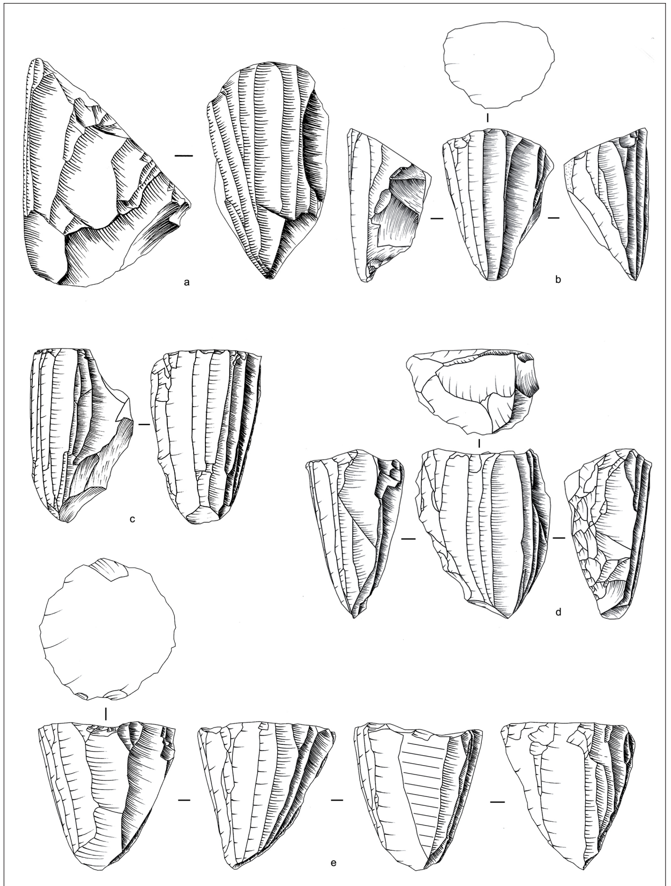
Figure S4. Amakomanak site (Alaska): a–e, microblade cores.
